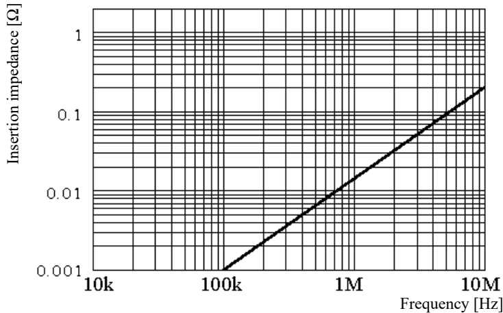
Figure 15 Insertion Impedance N2781B
